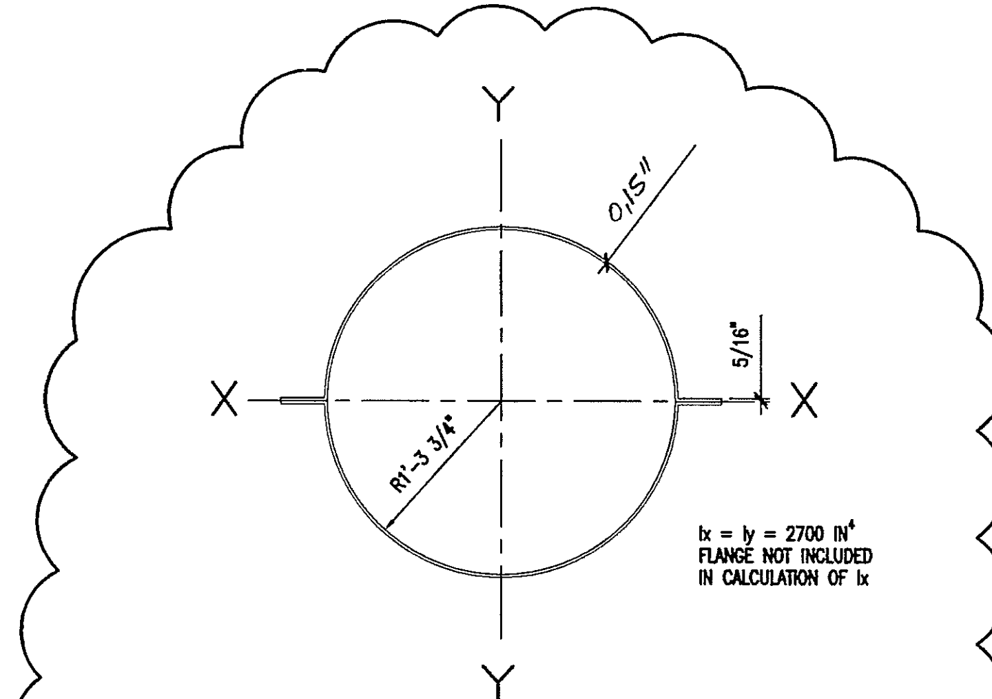
1 32" AQUATUBE SECTION PROPERTIES SCALE: 1"=1'-0"
