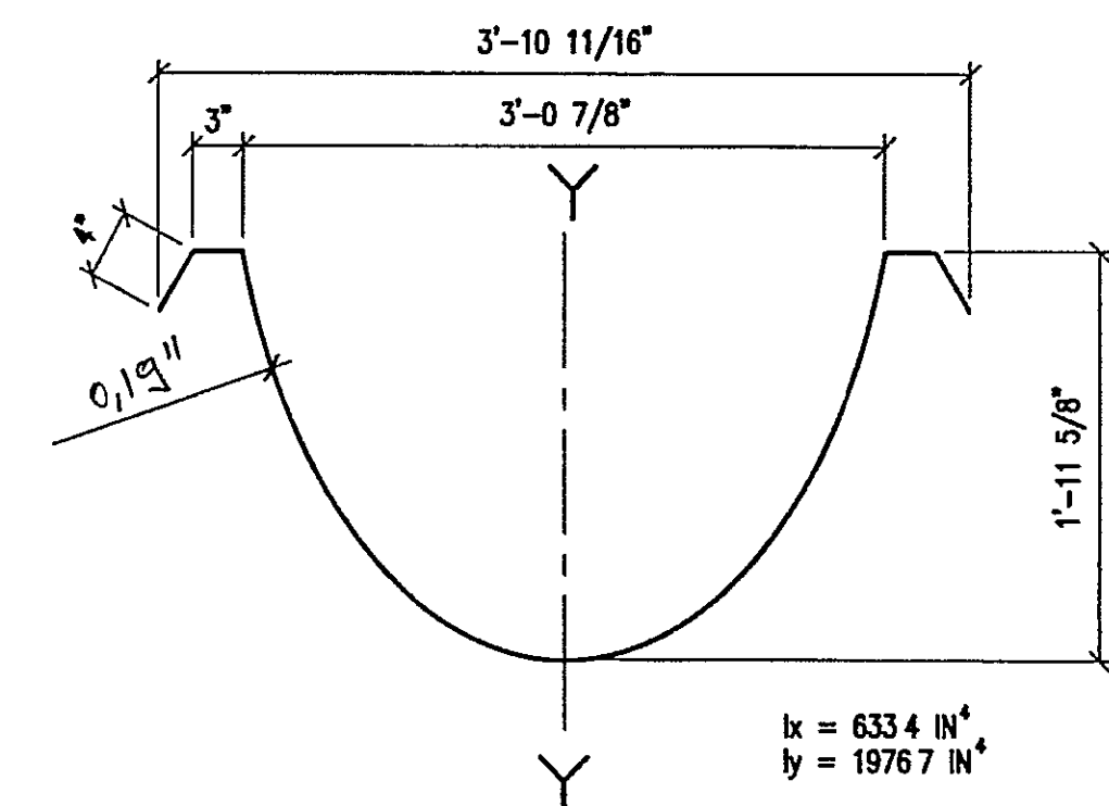
2 POOLSIDER SM SECTION PROPERTIES SCALE: 1"=1'-0"
